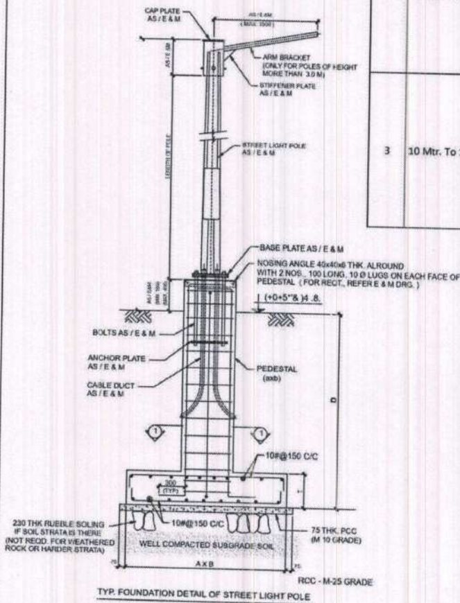
TYP. FOUNDATION DETAIL OF STREET LIGHT POLE
